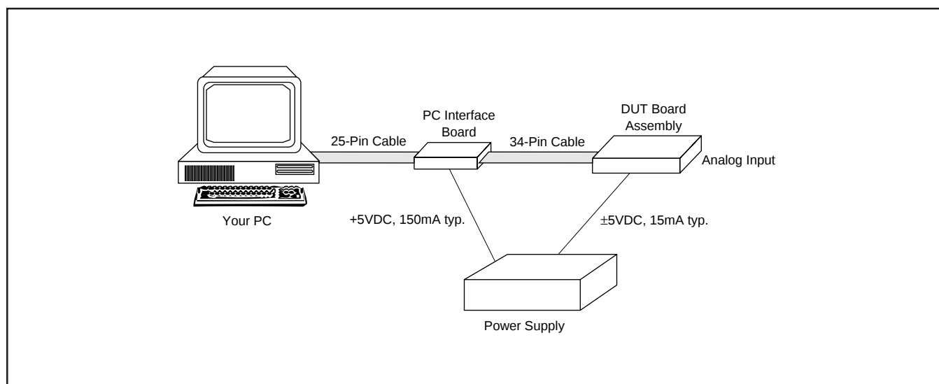
FIGURE 1. DEM-DDC112U-C Evaluation Fixture Connection Diagram.
